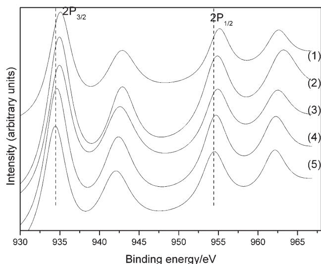
Figure 3. Cu 2p XPS region in the corresponding XPS spectra of (1) La-Cu-HTLcs, (2) Sm-Cu-HTLcs, (3) Y-Cu-HTLcs, (4) Ce-Cu-HTLcs and (5) Cu-HTLcs.
