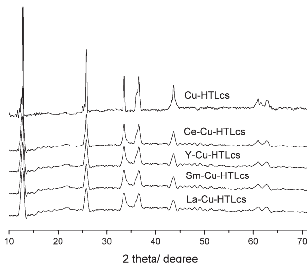
Figure 1. X-ray diffraction pattern of the copper-containing hydrotalcites.
