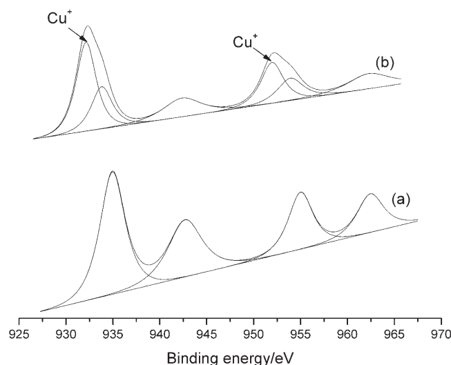
Figure 5. Comparison of Cu 2p XPS spectra of La-Cu-HTLcs before (a) and after (b) \text{H}_2\text{O}_2 treatment.
