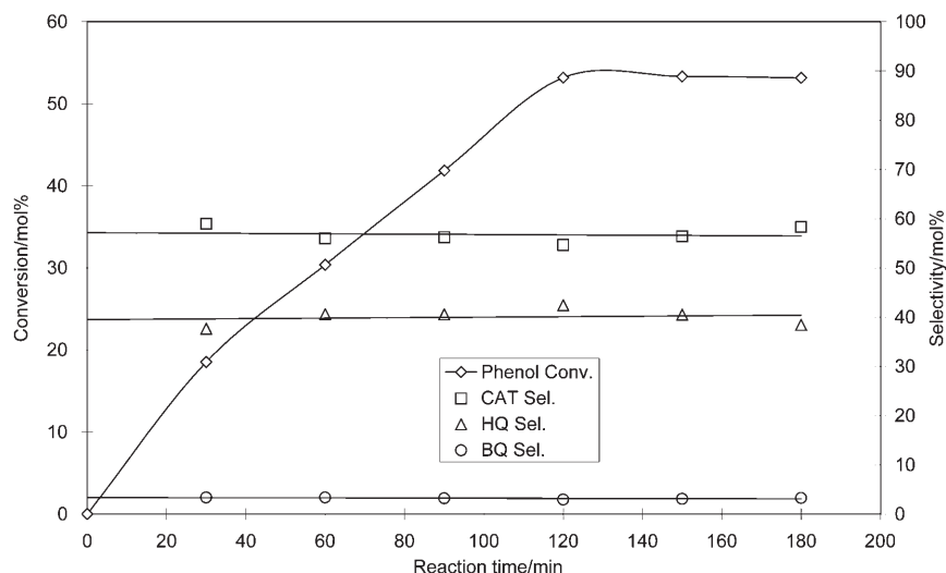
Figure 4. Effect of reaction time on phenol hydroxylation. Reaction conditions: 0.5 g phenol, 0.025 g La-Cu-HTLcs, 1 mL 30 wt % \text{H}_2\text{O}_2 solution, 10 mL distilled water, temperature 70^\circ\text{C} .
