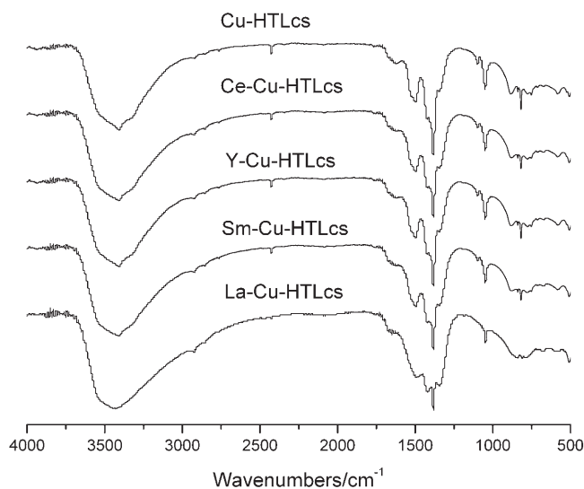
Figure 2. FT-IR spectra of the copper-containing hydrotalcites.
